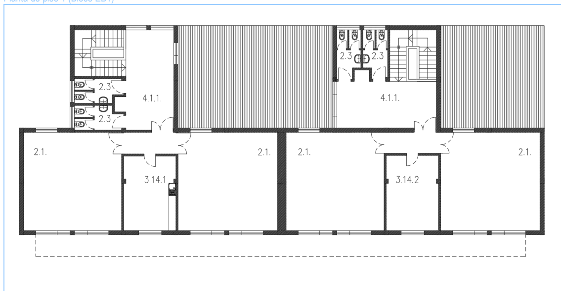
Planta do piso 1 (Bloco EB1)
