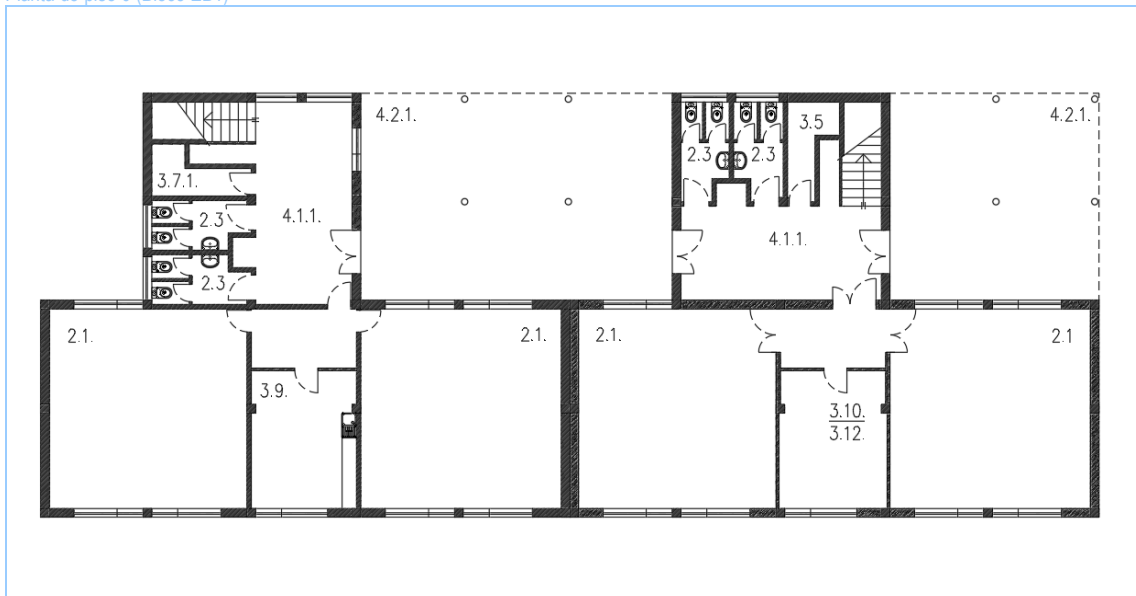
Planta do piso 0 (Bloco EB1)
